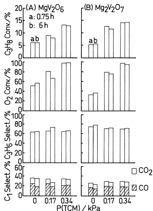
Fig. 3. Effects of P(TCM) on MgV_2O_6 and Mg_2V_2O_7 at 723 K. Reaction conditions: as in Fig. 1 except P(TCM) but Wt = 0.5 g.
