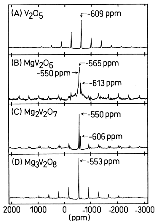
Fig. 2. ^{51}V MAS NMR of V_2O_5 (A), MgV_2O_6 (B), Mg_2V_2O_7 (C), and Mg_3V_2O_8 (D).
